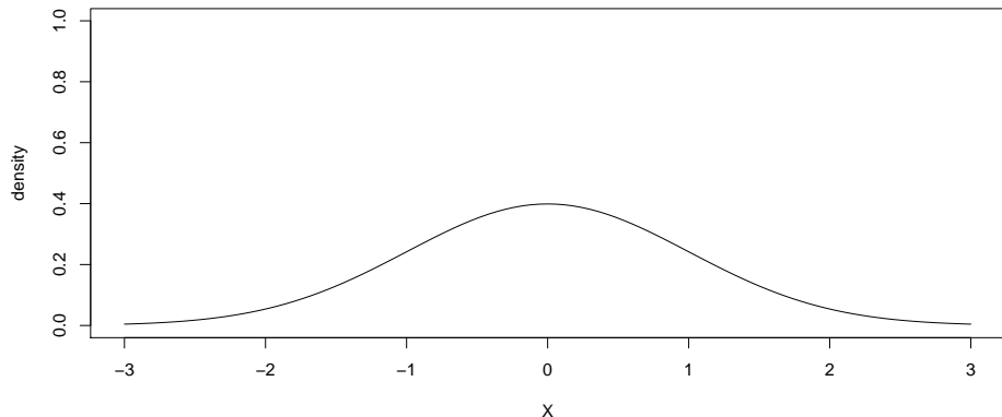
Normal density
